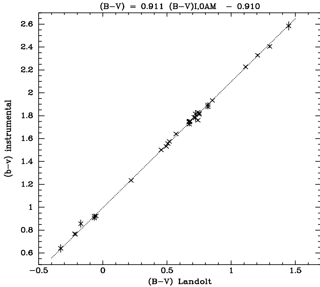
Figure 19.3: NURO B–V transformation. Note the large value of b , and the large offset between the numbers on the x and y axis.
