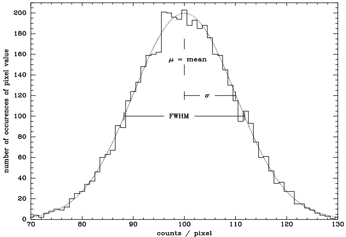
Figure 20.1: Histogram of photons falling on the pixels of a CCD. We assume the CCD is uniformly illuminated and that the CCD is “perfect” - i.e. each pixel is exactly the same. In this example the mean number of photons hitting each pixel is 100. The histogram shows (at least schematically) the distribution of the counts measured on a number of pixels of a single exposure of the CCD. The smooth dotted line is the “best fit” Gaussian. If we make repeated measurements of a single pixel, with steady (not varying with time) illumination, we would get a similar distribution. Note that this graph may look like a PSF plot, but this is a histogram, not a plot of something vs. position or time. Make sure you understand what is plotted (and why)!
