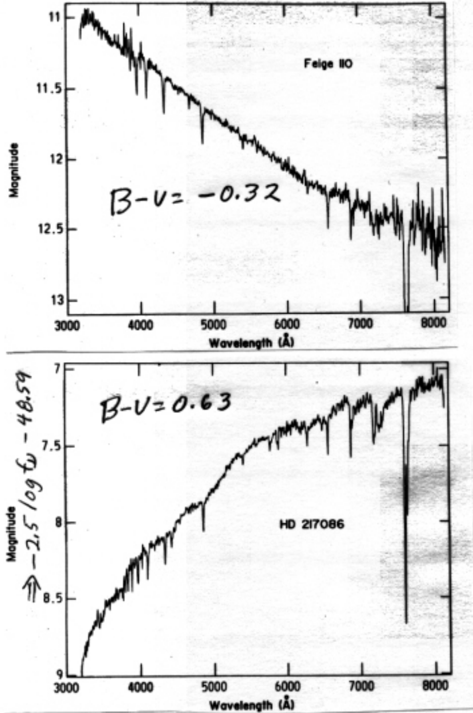
Figure 4.1: Spectrophotometry of a blue (top) and a yellow (bottom) star. The spectral resolution is about 50 \text{ \AA} , so the resolution is about 5000 / 50 = 100 . Note the connection between the slope of the graph and the color.
