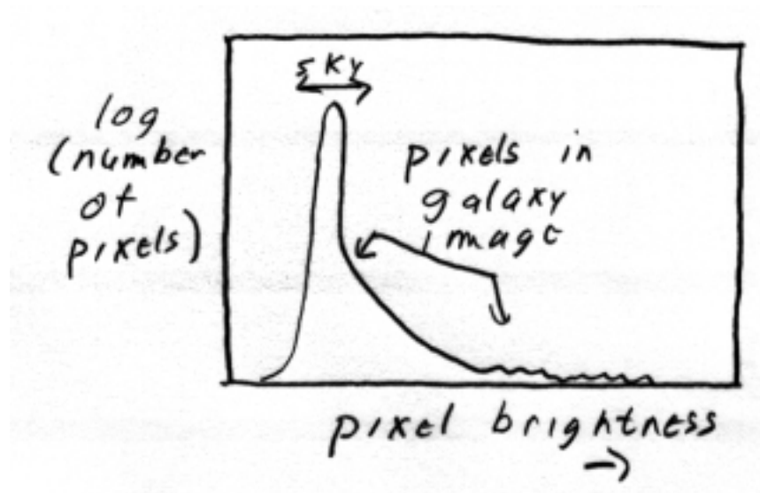
Figure 15.2: Histogram of a field largely filled with image of a galaxy. The galaxy pixels cover a smaller range of intensity than the star images, but a greater area of the chip. Many pixels in the outer parts of the galaxy are only a little above sky, so that the galaxy pixels blend into the sky pixels in the histogram.
