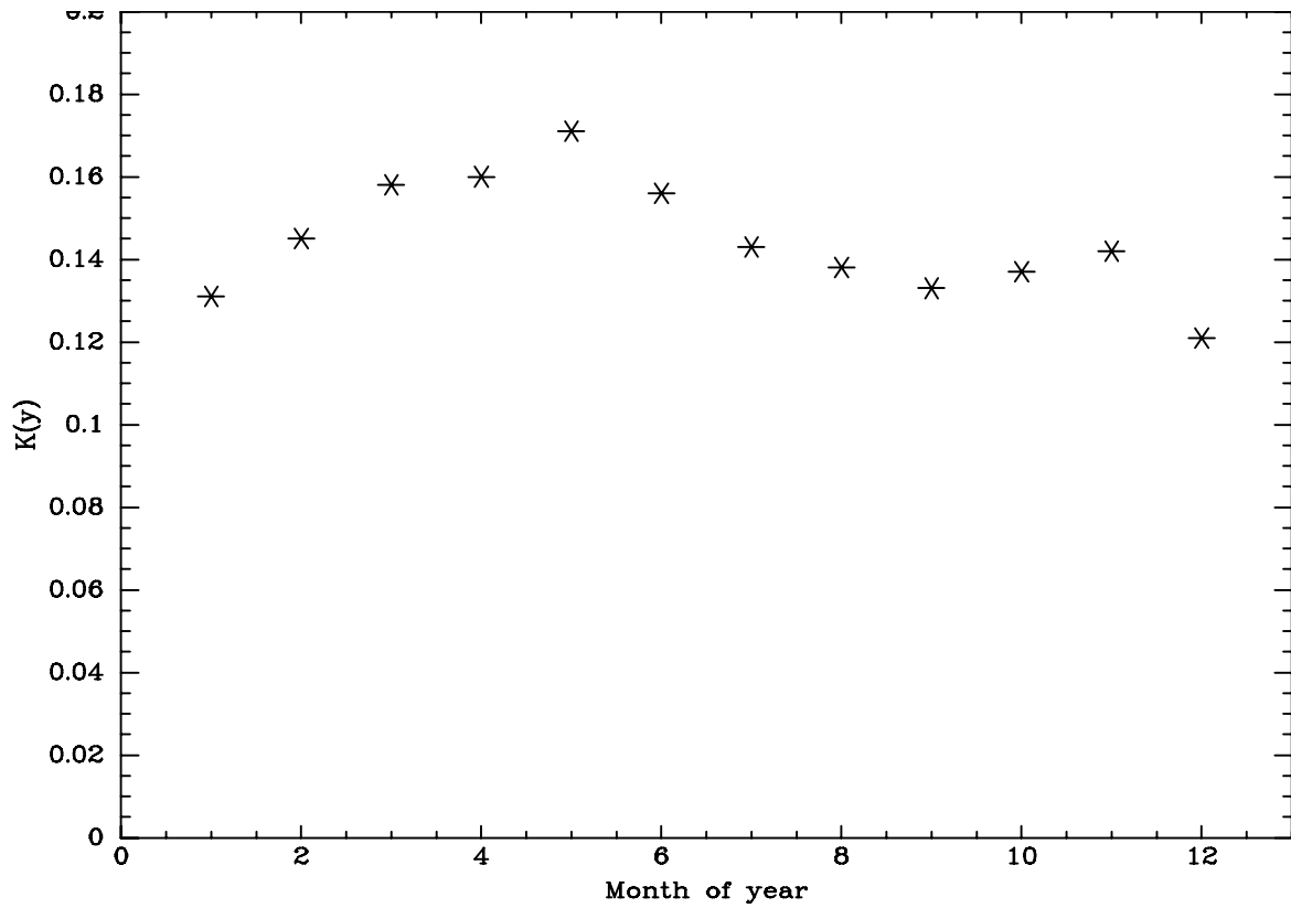
Figure 18.3: Seasonal variation of extinction over Flagstaff. Plotted are the monthly median extinction values (in mag) in the y band, an intermediate band filter centered at 5500 \text{ \AA} . These are for the years 1976-1980, when there was no significant volcanic contribution to the atmospheric extinction. Note that while there is a definite seasonal pattern, the individual nightly values (not shown here) show considerable night-to-night scatter. (data taken from G. W. Lockwood and D. T. Thompson AJ 92 p. 976 , 1986)
