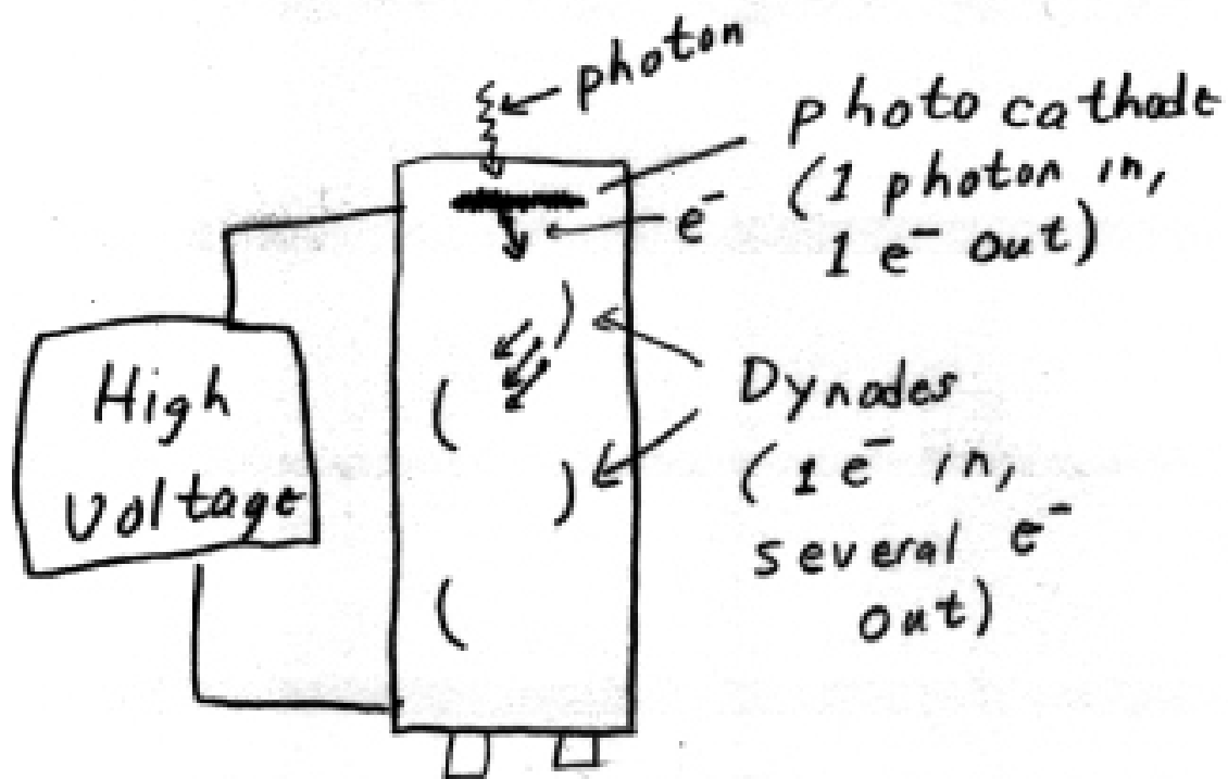
Figure 11.2: Schematic diagram of a photomultiplier tube (PMT). The high voltage supply creates an electric field that accelerates electrons along the tube. At each dynode, an impinging electron releases several electrons, which are then accelerated towards the next dynode, where each of them knock loose several more electrons. Through this cascade, a single photon hitting the photocathode releases an easily counted pulse of many electrons.
