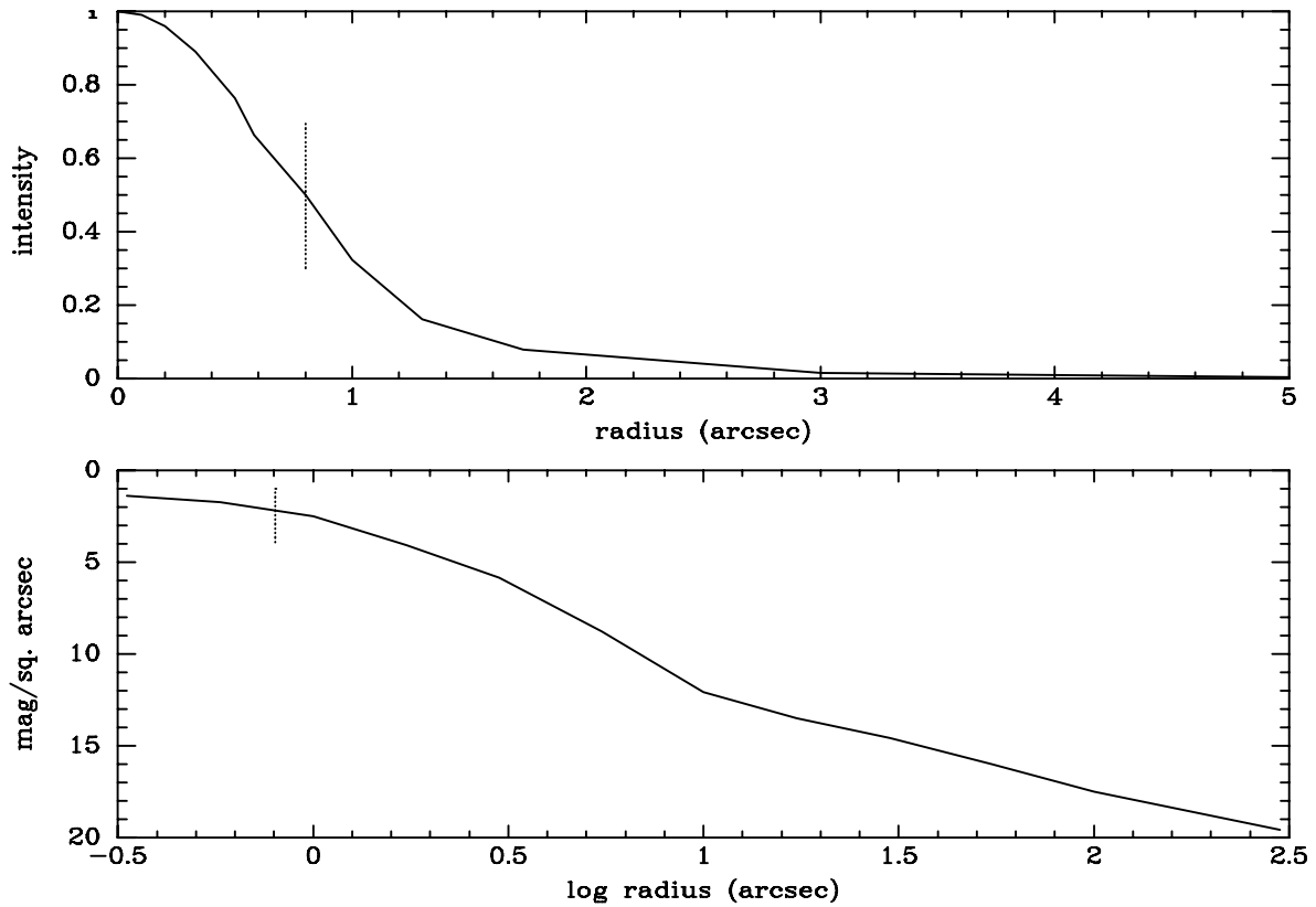
Figure 17.1: Typical Stellar Point Spread Function (PSF). This particular PSF is of a star in seeing of about 1.6 arcsec FWHM (King PASP 83, 199, 1971). Top panel: Radial intensity of light (normalized to center= 1.0) for this PSF. On this plot, the HWHM, the radius at which the PSF drops to half its central or peak value, is marked by the vertical dotted line. Bottom panel: This is a plot of surface brightness (mag/ sq. arcsec) (essentially logarithm of intensity) vs. logarithm of radius from the center of the image. The HWHM is again marked by the vertical dotted line. Note that the lower panel shows the PSF to a much larger radius (out to over 300 arcsec) than shown in the top panel (5 arcsec). The logarithmic y axis allows us to see the very faint outer regions of the PSF at large radii that would be invisible in the top panel linear intensity display. Note that the PSF simply fades out- there is no sharp edge where the PSF reaches zero intensity.
