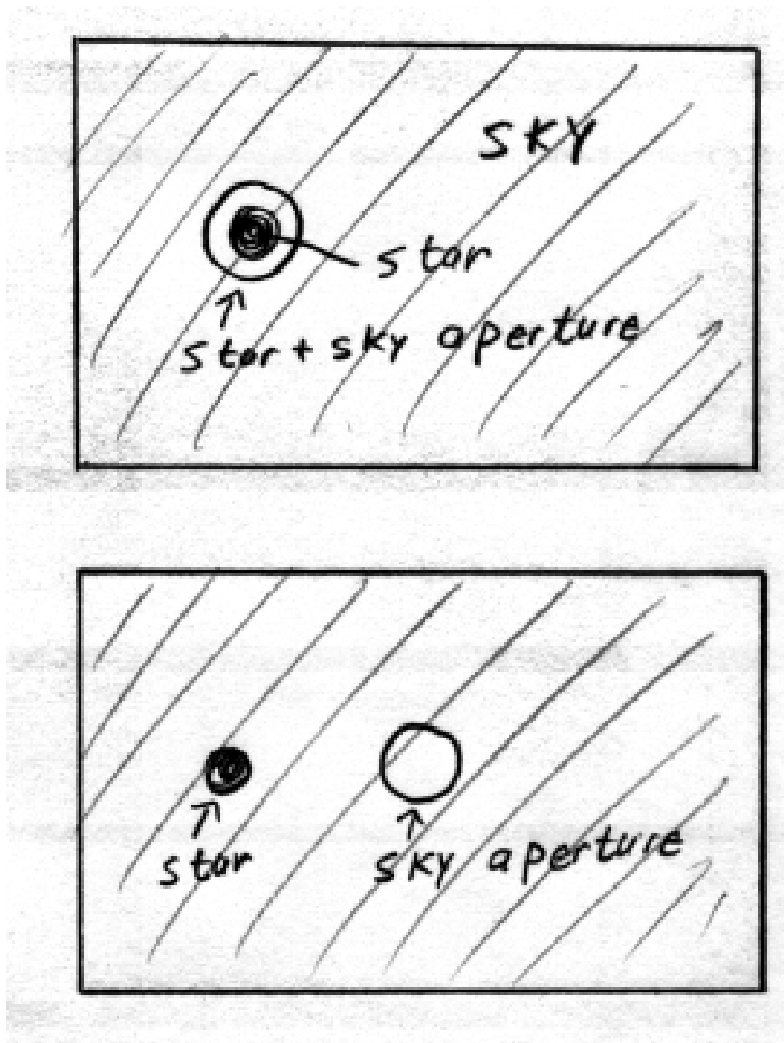
Figure 20.2: Sky+star aperture and sky aperture. This is the simple “photometer model” of measuring the sky background, as the star+sky and sky are measured with the same circular aperture. As discussed elsewhere, a CCD allows us to use other measurement apertures to measure the sky (such as a sky annulus around the star being measured).
