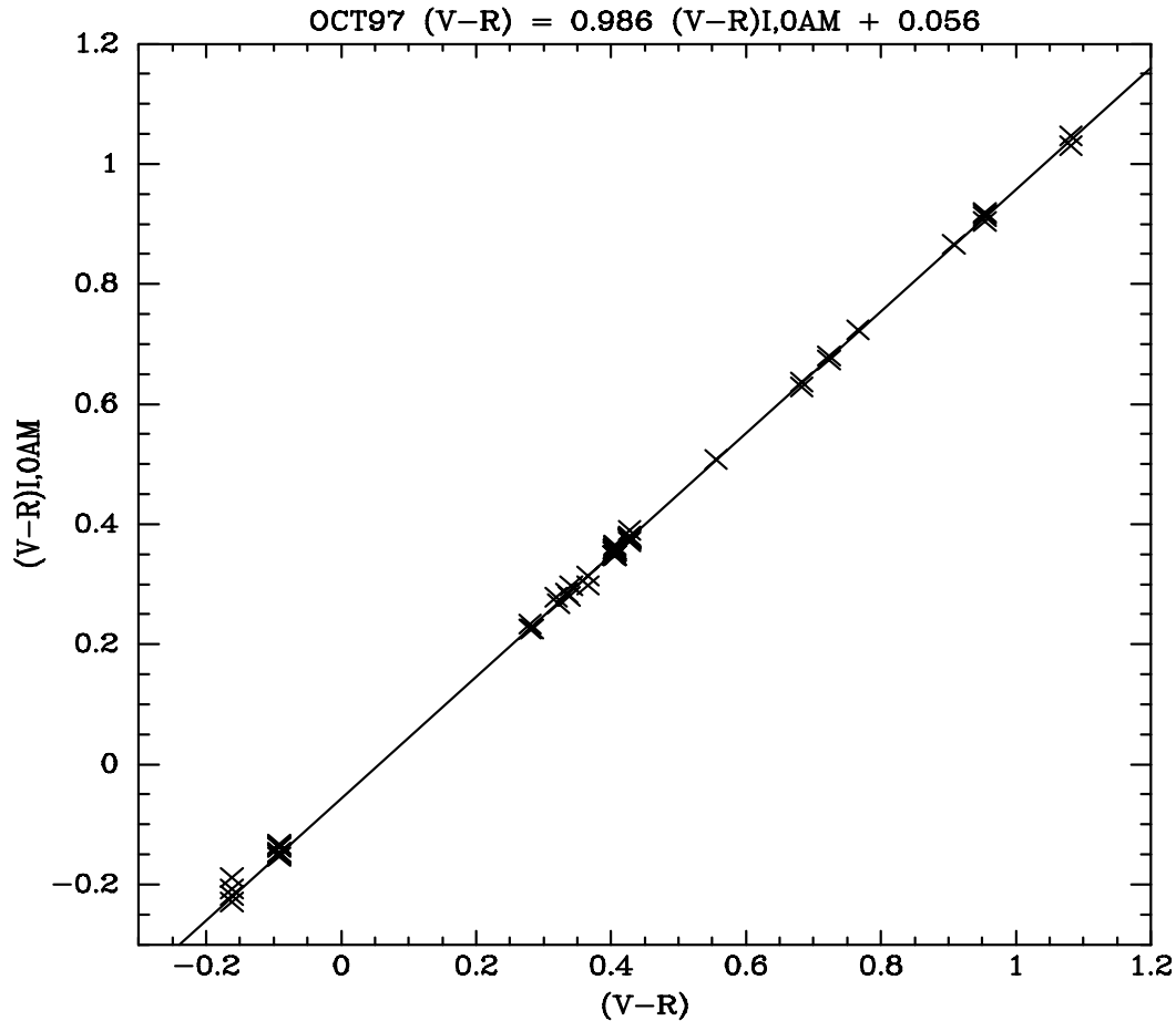
Figure 19.1: Steward 2.3m V–R transformation. Plotted on the x axis are the standard (Landolt) V–R colors of standard stars. Plotted on the y axis are the instrumental colors, corrected to zero airmass. The title gives the transformation equation. The sharp-eyed among you may see that the fit does not seem to be quite right for the two bluest sets of points. This is because the fit was done to deemphasize these points, as none of the objects we were interested in were anywhere near this blue.
