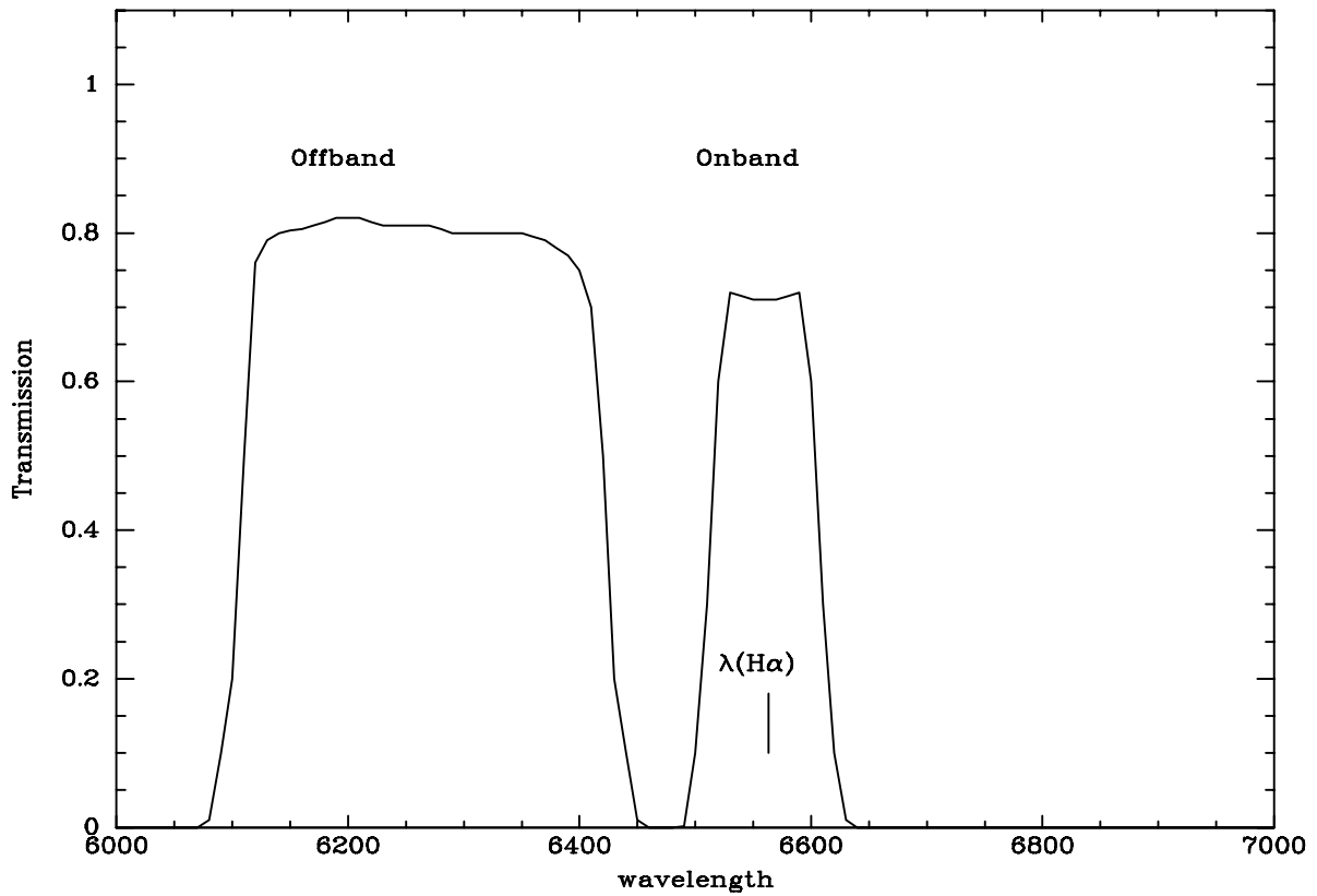
Figure 22.2: The passbands of a typical set of filters used to image \text{H}\alpha radiation. The onband filter passes \text{H}\alpha and continuum, while the offband filter only passes nearby (in wavelength) continuum light. When observing external galaxies, a set of onband filters with different central wavelengths is used for galaxies in different redshift ranges, as the observed wavelength of \text{H}\alpha is different for galaxies of different redshifts. These filters would be interference filters, not colored glass like the V filter in the previous figure.
