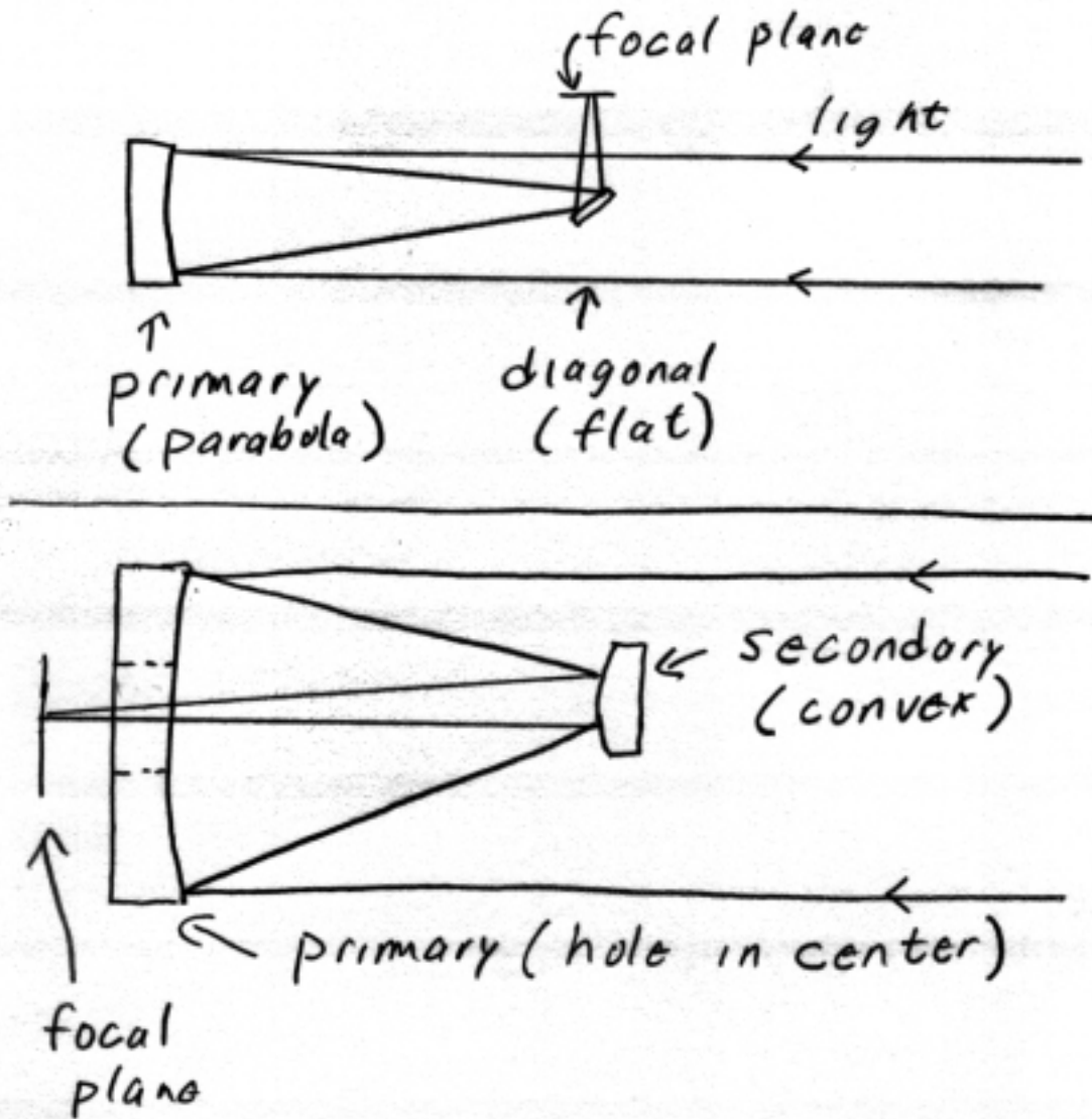
Figure 5.2: Top: Newtonian ; bottom: Cassegrain or RC system. In these types of systems, the diagonal or secondary is usually held in place by 4 vanes attached to the inside of the telescope structure. Diffraction effects from light passing by these vanes are responsible for the familiar lines seen emanating from bright stars on many images of the sky. These lines are called “diffraction spikes”.
