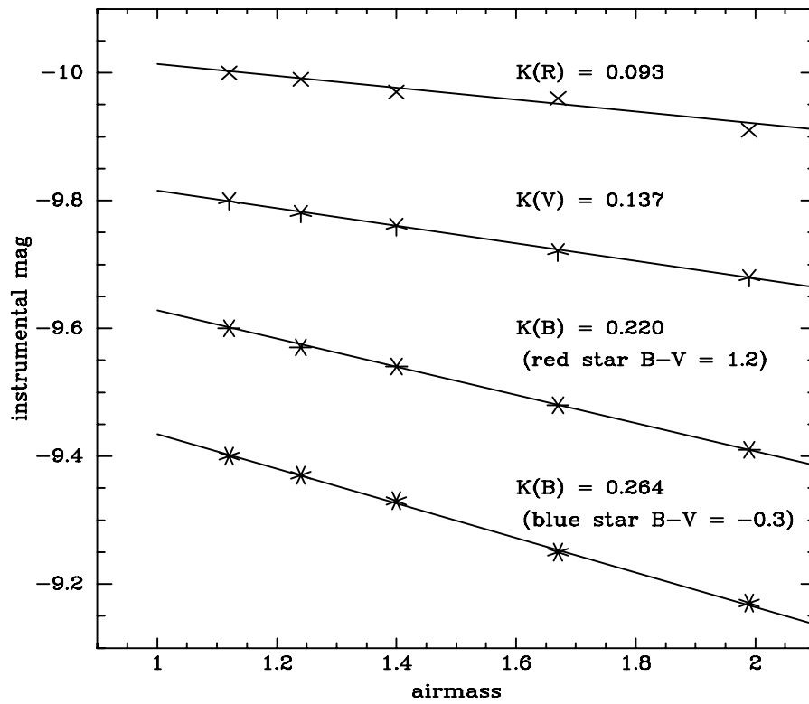
Figure 18.1: Instrumental mag vs. airmass for a star. This shows that the K value is the slope of the line in the mag vs. airmass plot. The instrumental magnitudes have been arbitrarily shifted so they would not overlap. An exercise for the student: from the information on the B extinction for two stars as shown on the graph, calculate K'_B and K''_B .
