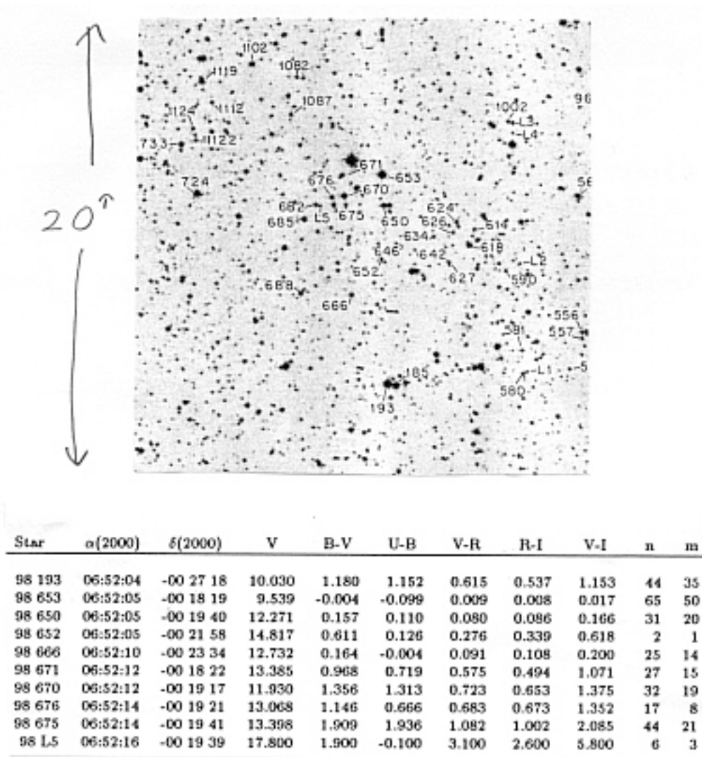
Figure 23.1: Top: A portion of the SA98 field finding chart from Landolt article. The field shown is about 20 x 20 arcmin. Bottom: Small portion of table from Landolt article. Columns are mostly self-explanatory, except for n , which is number of times each star was observed; and m , which is number of different nights each star was observed. The table also shows mean errors for each quantity for each star, but these have been omitted for clarity.
