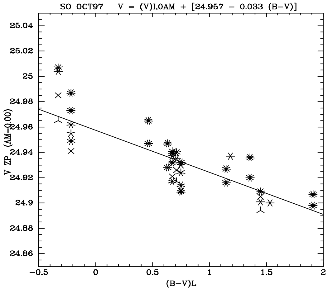
Figure 19.2: Steward Observatory 2.3m telescope V transformation. Different symbols are for different nights during the run. There is a slight color dependence to the V mag zero point. The transformation equation is shown in the title.
