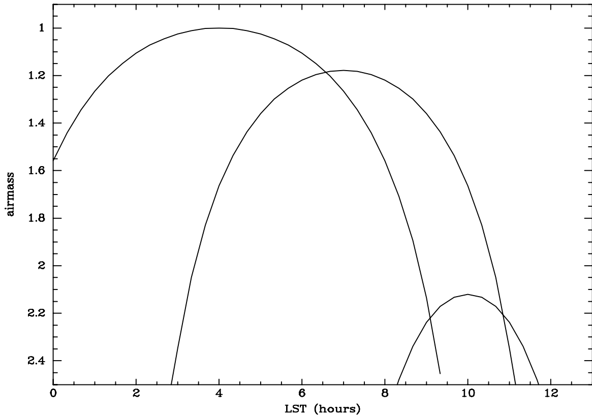
Figure 26.3: Example airmass vs. time plot for observing at Kitt Peak (latitude = 32 degrees). The first object to transit is at a declination equal to 32 degrees, so transits at the zenith at 1.0 airmass. The next object transits 32 degrees south of the zenith (say a Landolt field on the equator, dec = 0 degrees). The third object is at declination = -30 degrees, which is pretty far south to be observing from Kitt Peak, as the object never gets higher in the sky than airmass 2.1.
