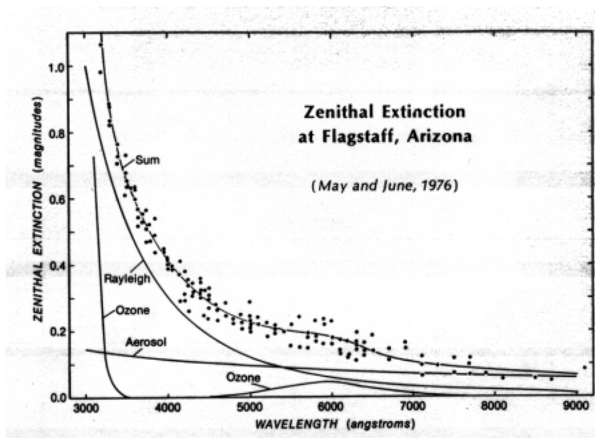
Figure 18.2: Extinction looking “straight up” from Flagstaff, showing components of extinction. (from “A New Absolute Calibration of Vega” Sky and Telescope Oct 1978)
