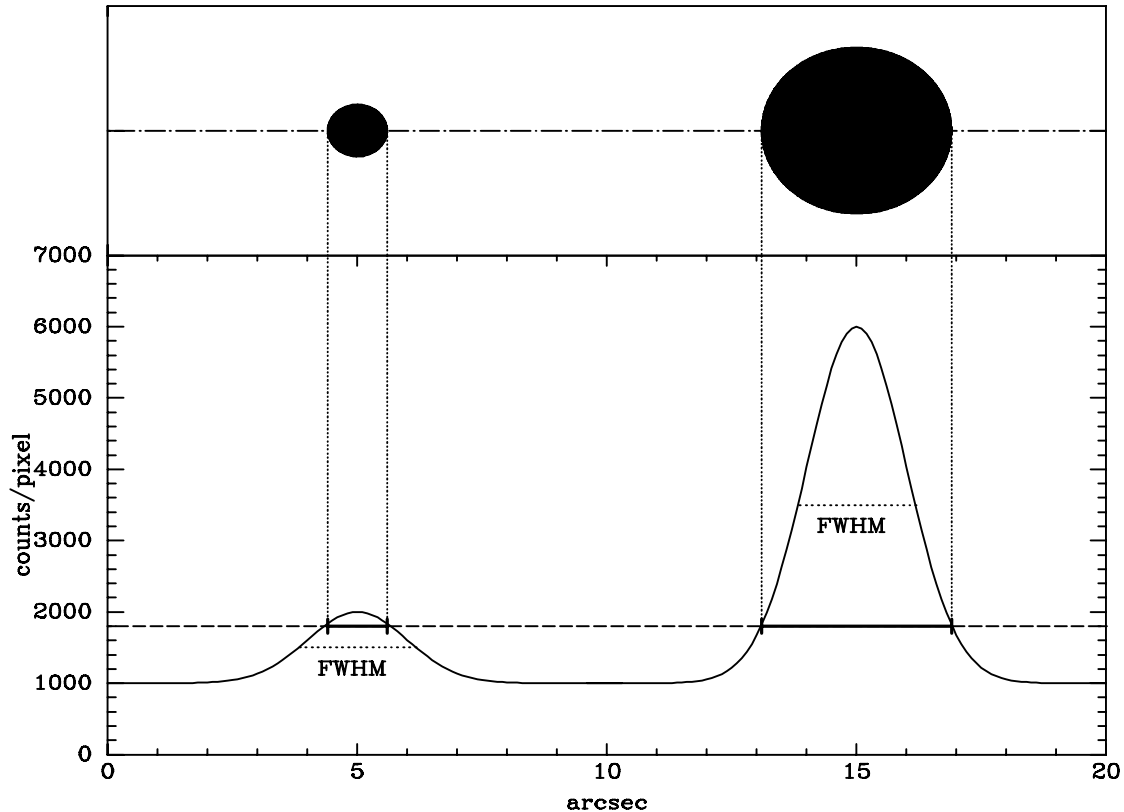
Figure 17.2: Why bright stars look bigger than faint stars, even though all stars have same image shape and size. Top: Very schematic image of a faint star and a bright star (bright star 5 times flux of faint star), showing brighter star looking bigger than fainter. This “image” maps all pixels with value less than 1800 to white, and all above 1800 to black. (Ignore the slight ellipticity of the stars.) Bottom: Brightness profile along dot-dash line crossing the centers of the two stars. The shapes of the two stars are exactly the same, the bright star is simply 5 times the intensity above sky at each point relative to the faint star. Brightness along the dashed line at constant level of 1800 counts/ pixel across image shows that, while the bright and faint star have the same shape (same PSF), the bright star looks bigger at each gray level on the image. The dotted line on each star profile marks the FWHM of each star (here the FWHM is about 2.3 arcsec). The solid line intersecting each profile at counts/ pixel = 1800 shows the size of the star on the “image” in the top panel. Note: In a real CCD image and plot, you would be able to see the individual pixels, so that the edge of the star image would be a set of squares, and the intensity profile along a single line would show a “stair step” pattern of individual pixels.
