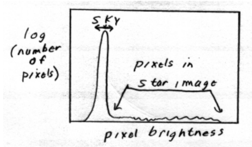
Figure 15.1: Histogram of a sparse star field. Because the star images cover a wide range of pixel intensity, but a small fraction of the image area, the star pixels are few in number but span a wide pixel brightness range.
