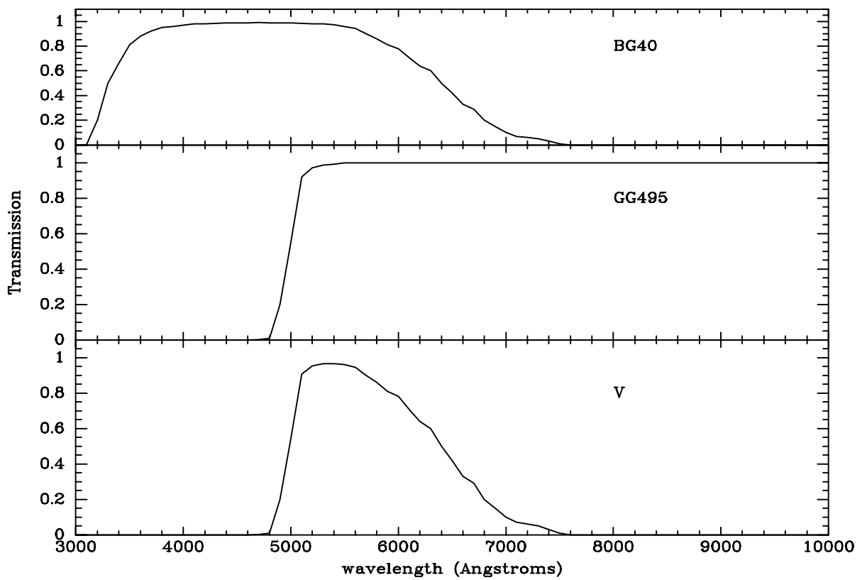
Figure 22.1: The transmission of a typical V filter, made up of two pieces of colored glass. Top: the transmission curve of a piece of BG40 glass. Middle: the transmission curve of GG495 glass. Bottom: The transmission curve of the V filter made up of the two pieces of glass together.
